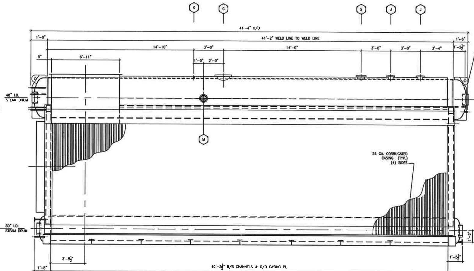
SIDE WALL BOILER 9201 AS SHOWN BOILER 9301 OPP. HAND
