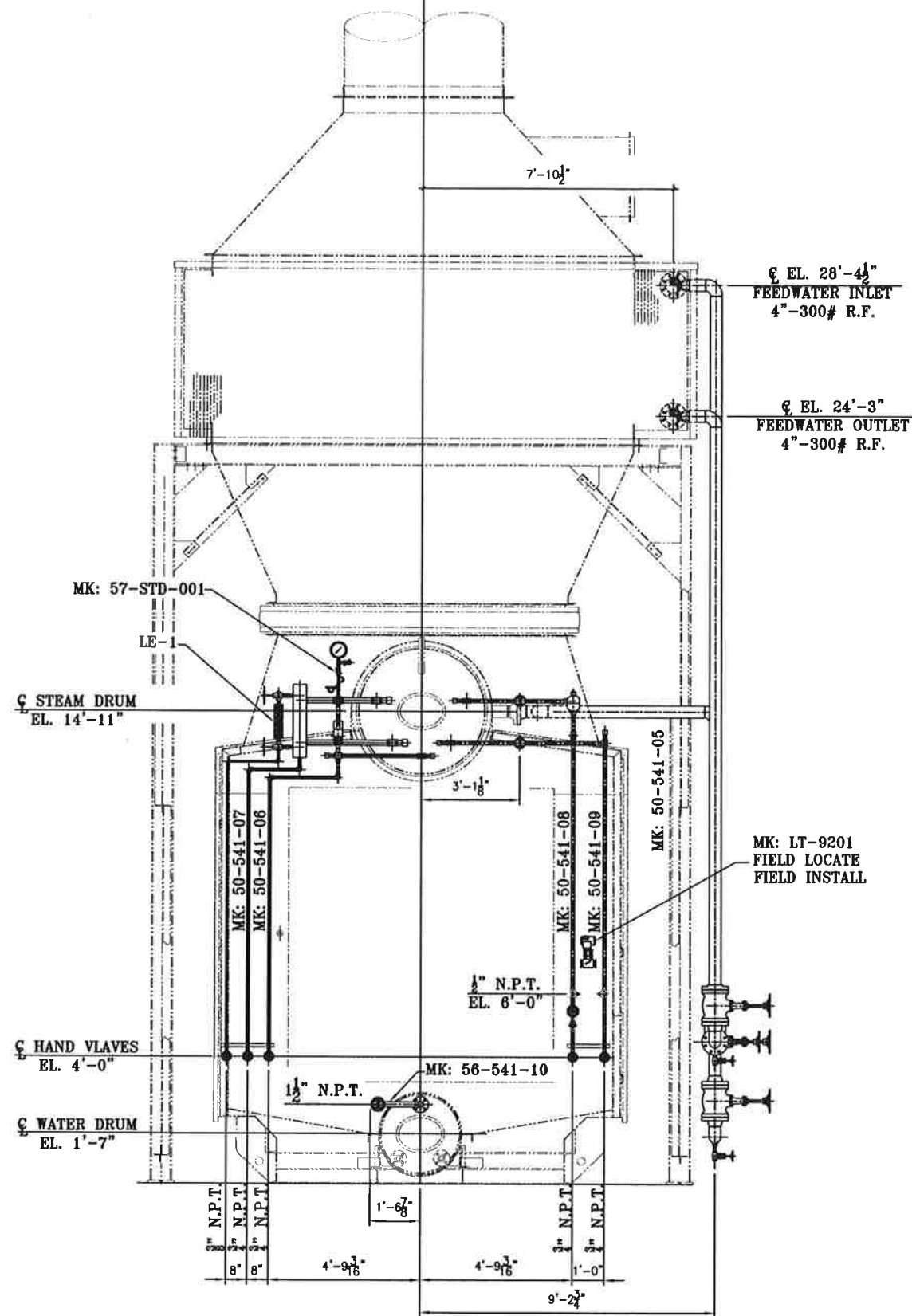
VIEW "A-A" BOILER (9201)
